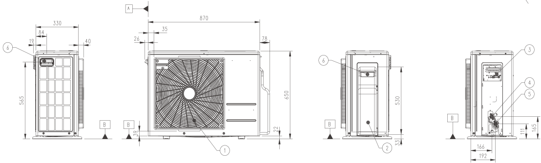
Side View (removed valve cover)
