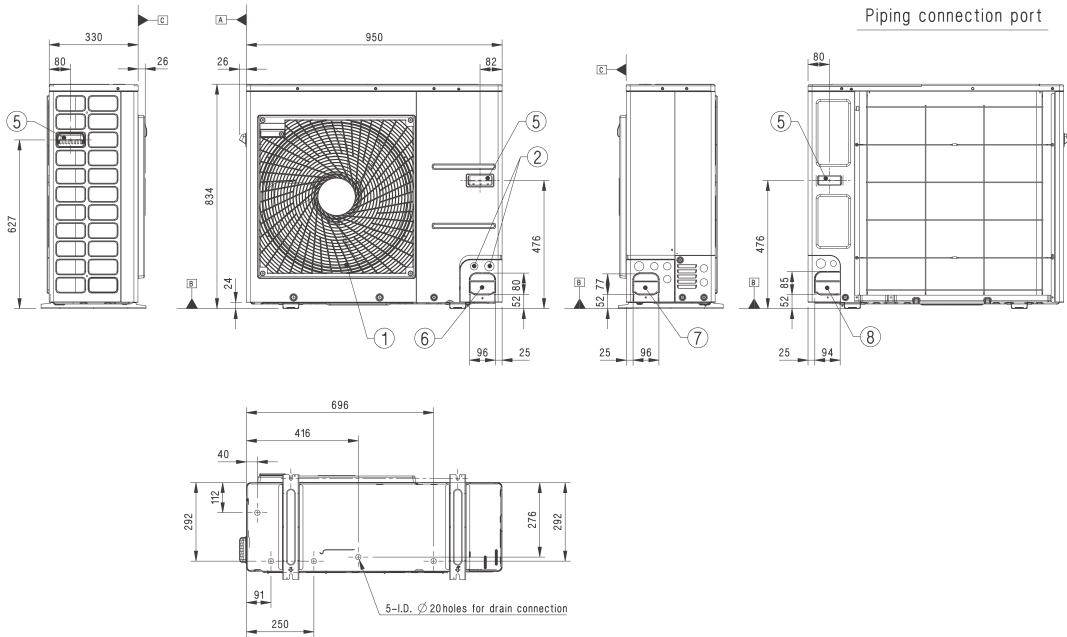
Piping connection port
